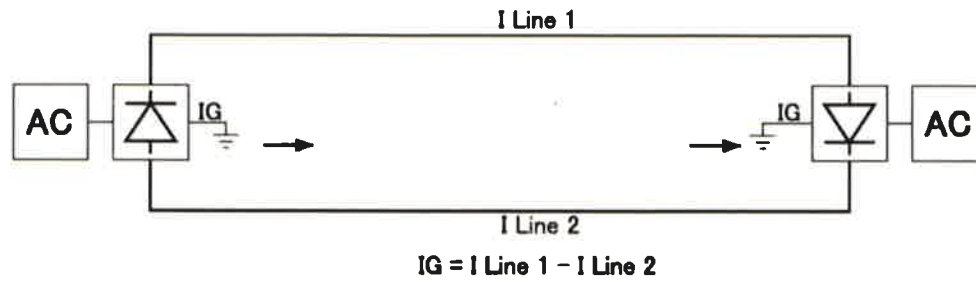
Figure 6. Bipole System (34)
