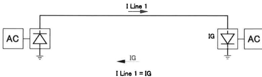
Figure 5. Monopole System (34)
